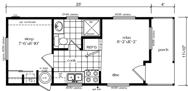
Optional layout, full porch, 292 Sq. Ft.
